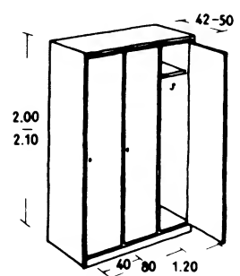
⑮ Cupboard for employees' clothing
